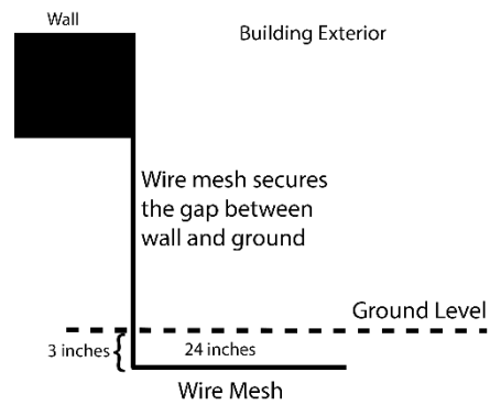
Figure 7. Diagram showing how to prevent skunk entry under a structure.
