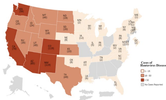
Figure 13. Hantavirus cases in the U.S. through 2021.
